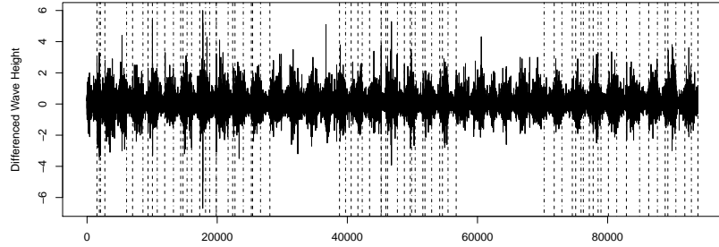
(c) Differenced Data with Binary Segmentation changepoints
