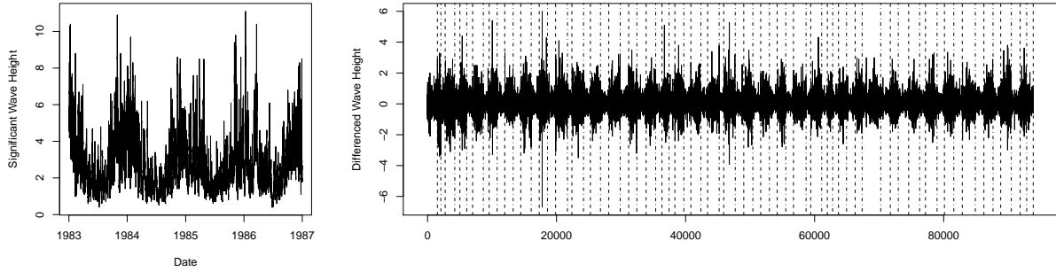
(a) Part of the original data
