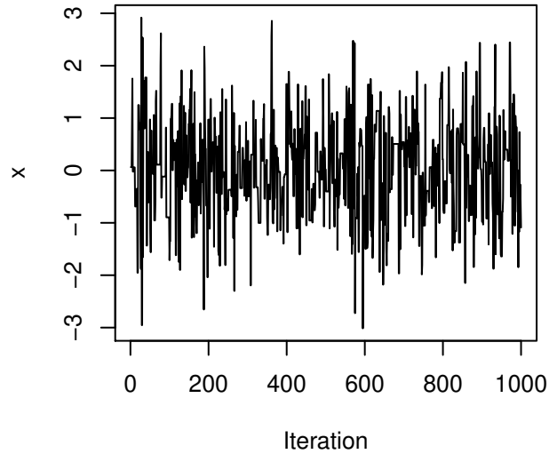
Indep. Samp.
