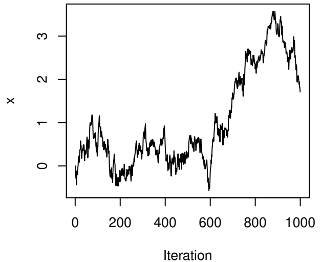
RWM N(0,0.01)
