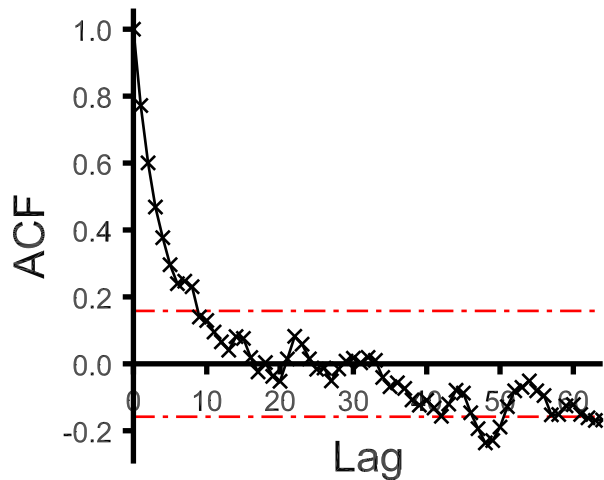
Sample autocorrelations
