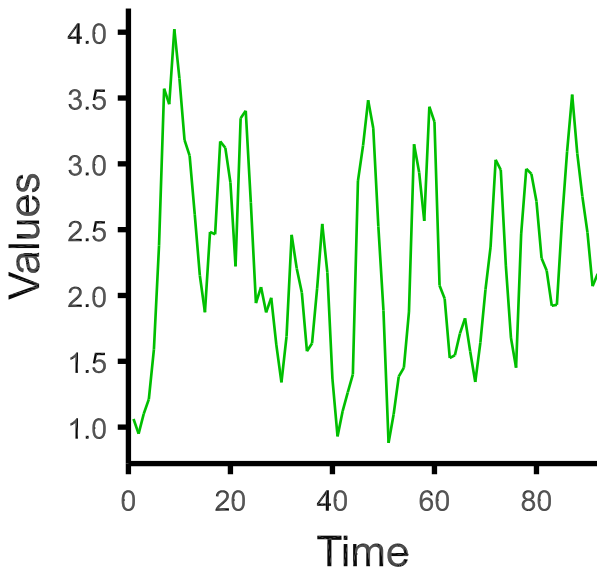
Time series: Ocean core isotope
