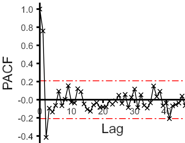
Sample partial autocorrelations
