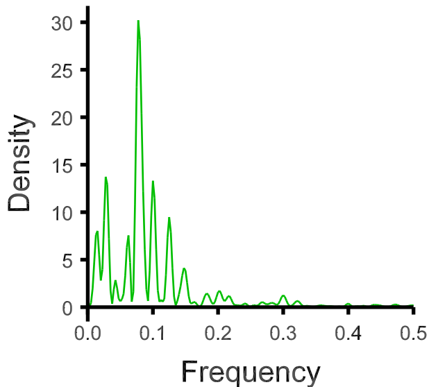
Sample spectral density
