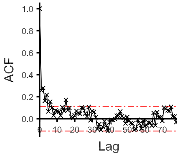
Sample autocorrelations
