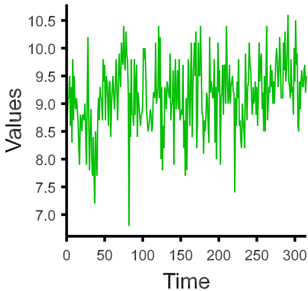
Time series: Annual average temperatures
