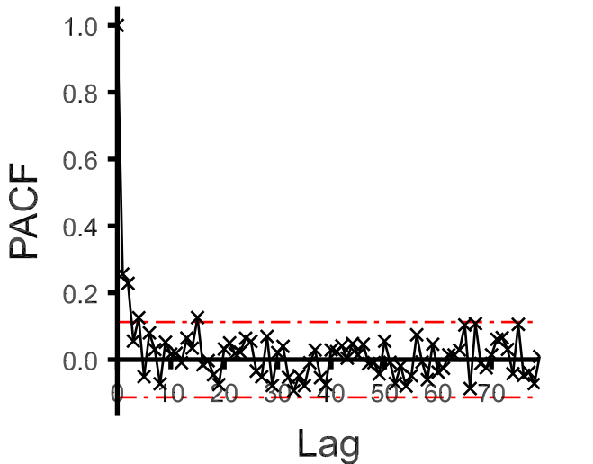
Sample partial autocorrelations
