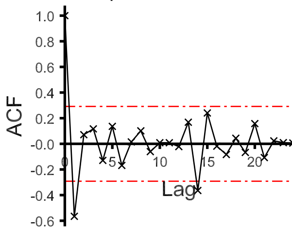
Sample autocorrelations
