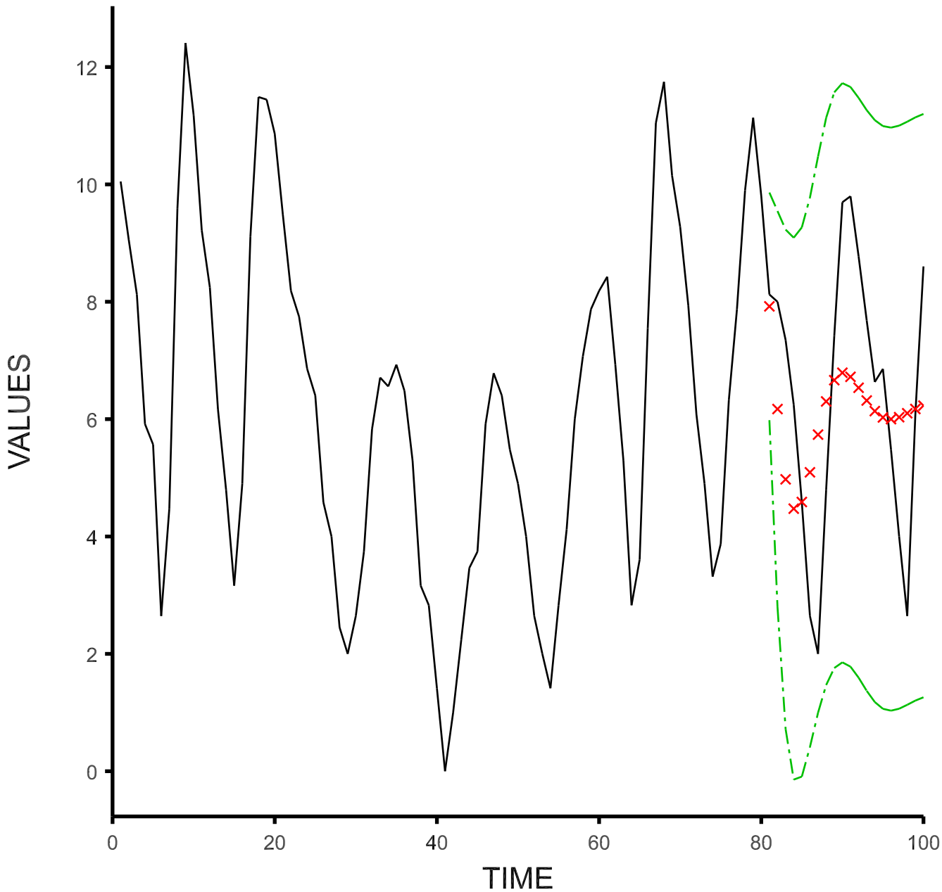
Series and forecasts with limits: Annual Sunspots
