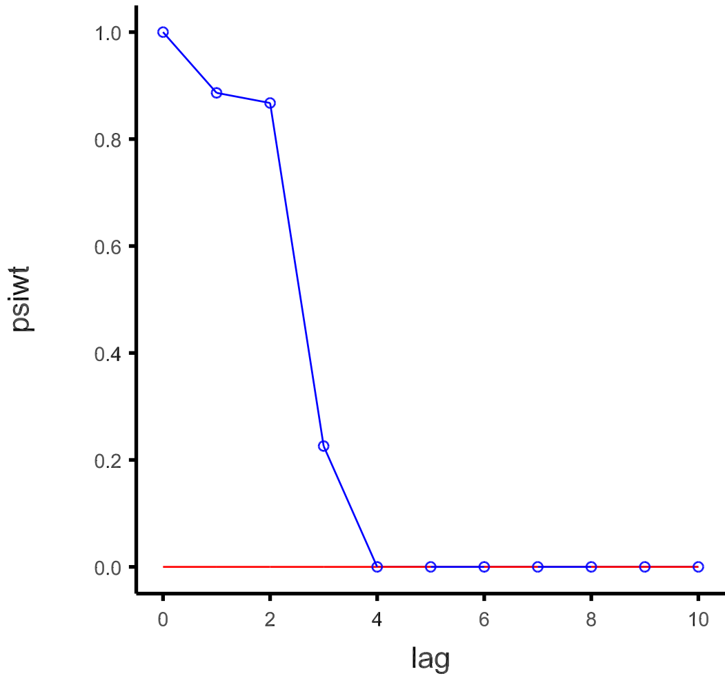
MA(3) model psi-weight
