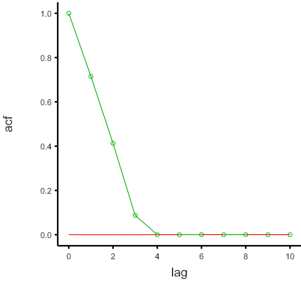
MA(3) model acf
