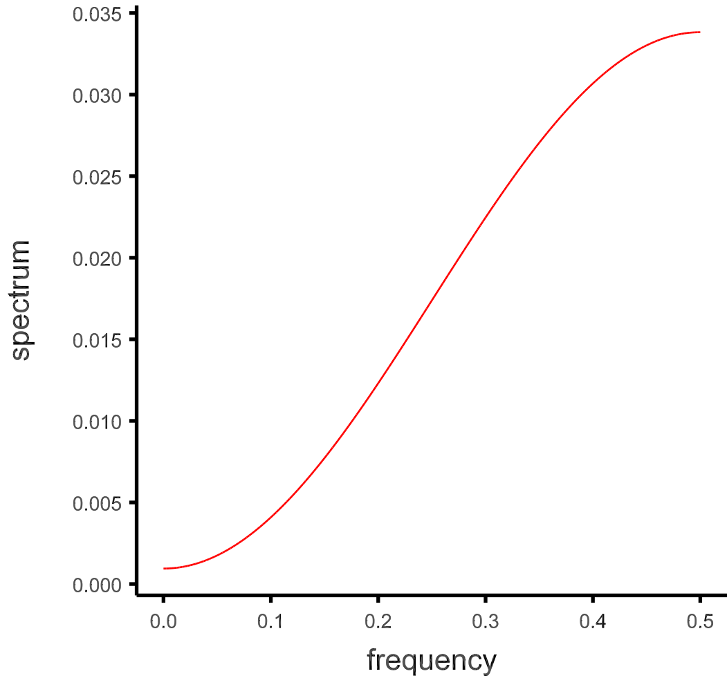
MA(1) model spectrum
