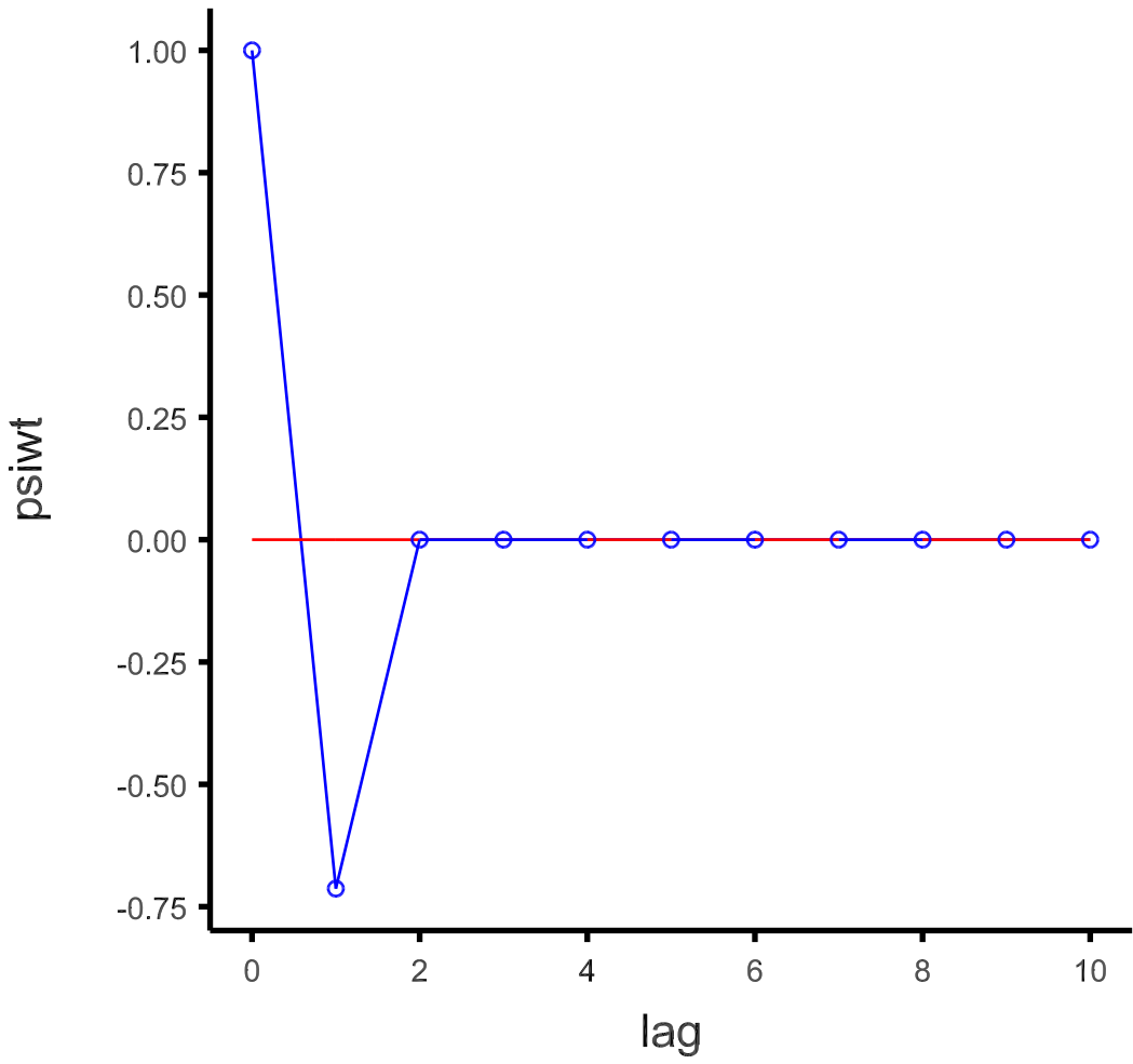
MA(1) model psi-weight
