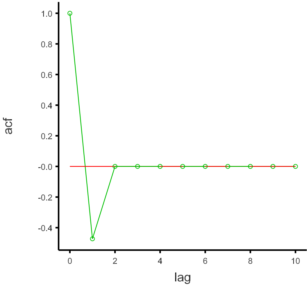
MA(1) model acf
