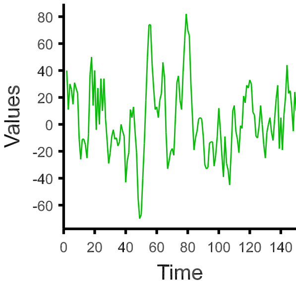
Time series: Changes in daylength
