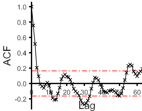
Sample autocorrelations
