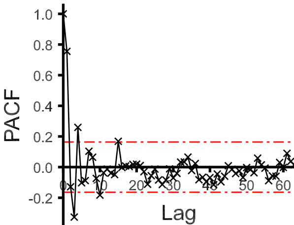
Sample partial autocorrelations
