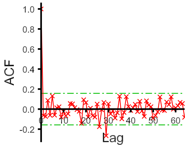
Sample autocorrelations
