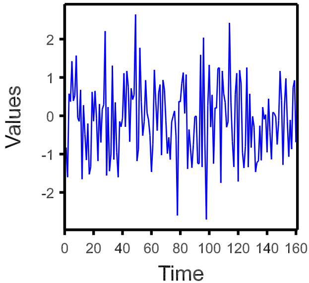
Time series: random
