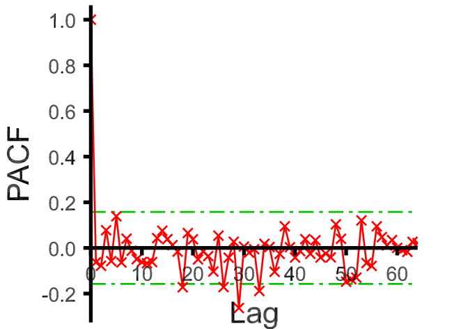
Sample partial autocorrelations
