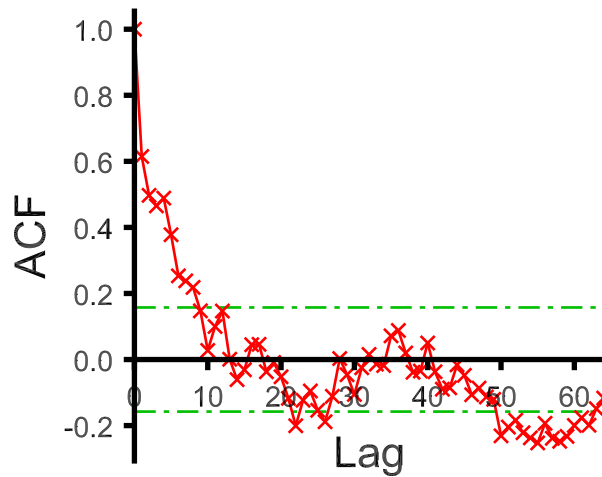
Sample autocorrelations
