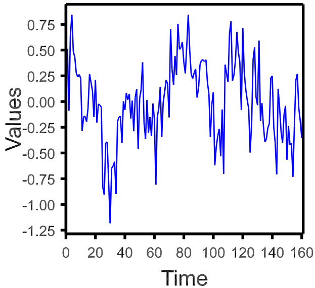
Time series: res
