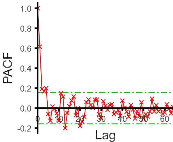
Sample partial autocorrelations
