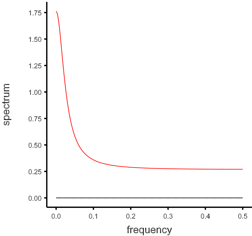
ARMA(1,1) model spectrum
