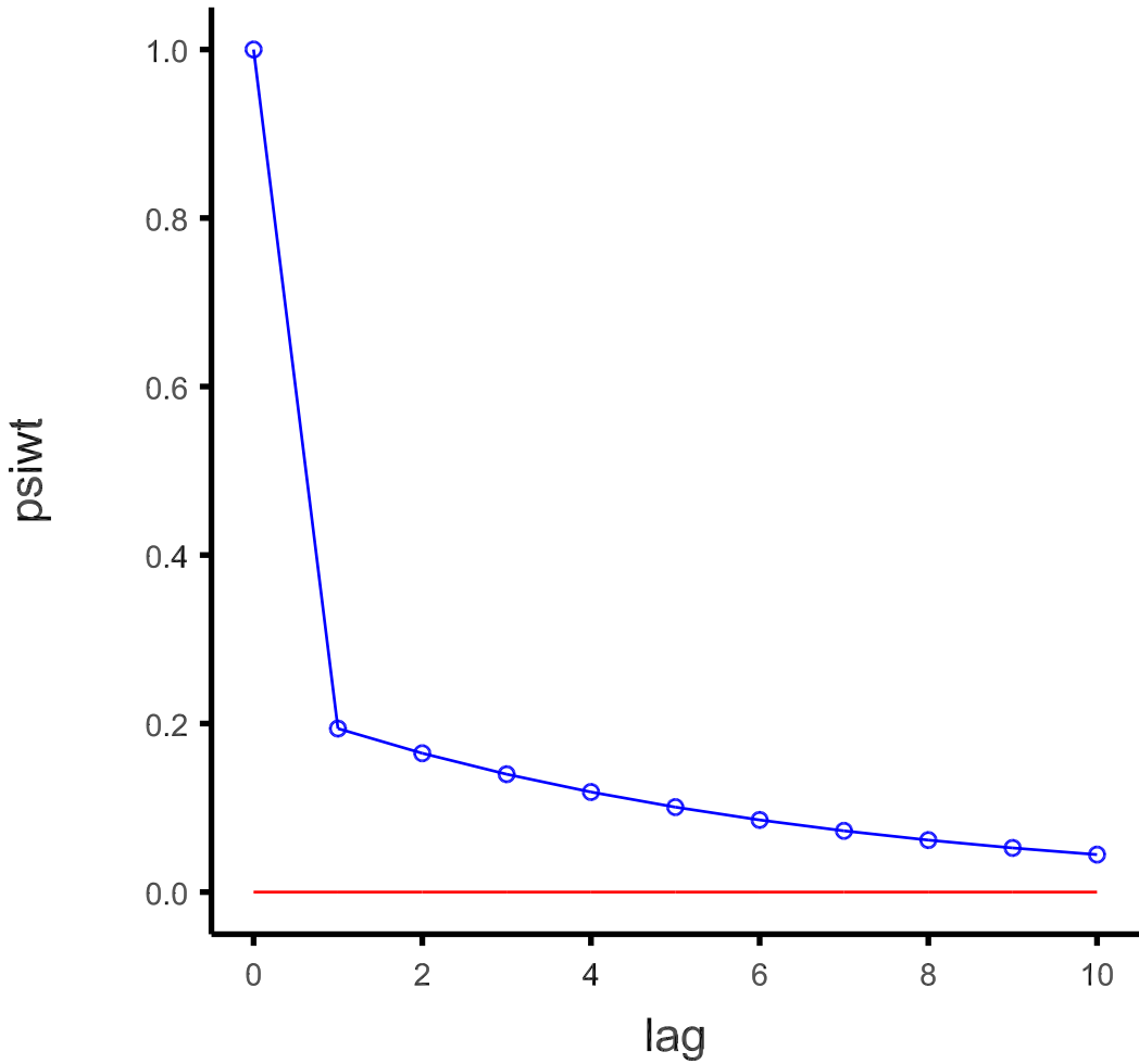
ARMA(1,1) model psi-weight
