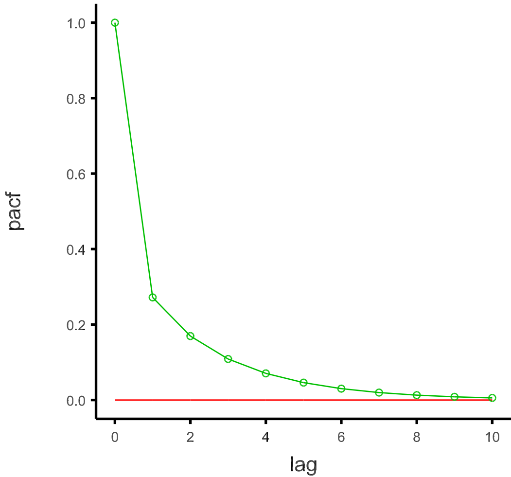
ARMA(1,1) model pacf
