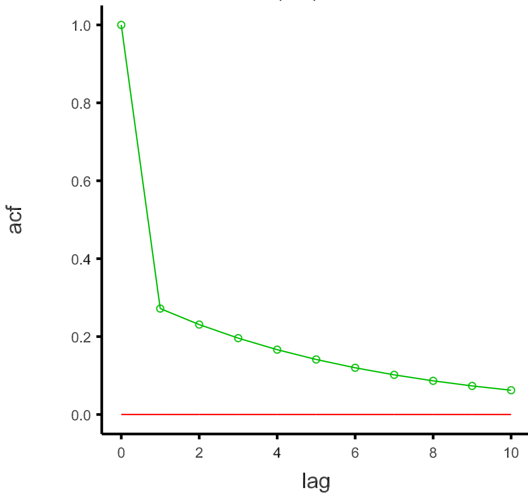
ARMA(1,1) model acf
