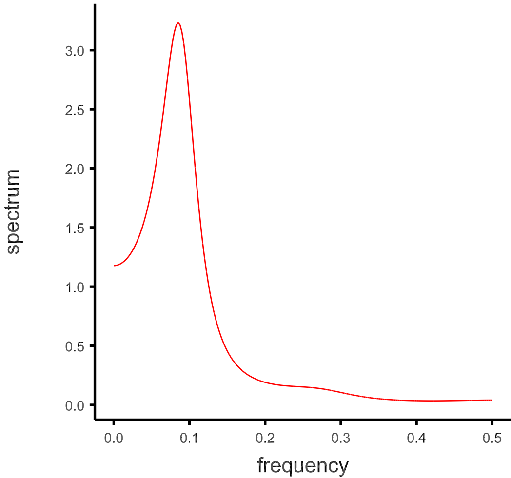
AR(6) model spectrum
