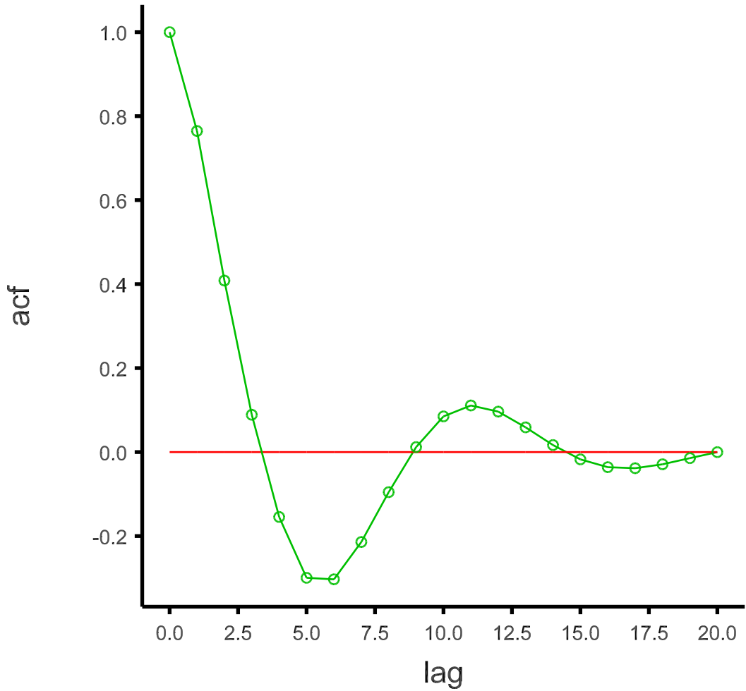
AR(6) model acf
