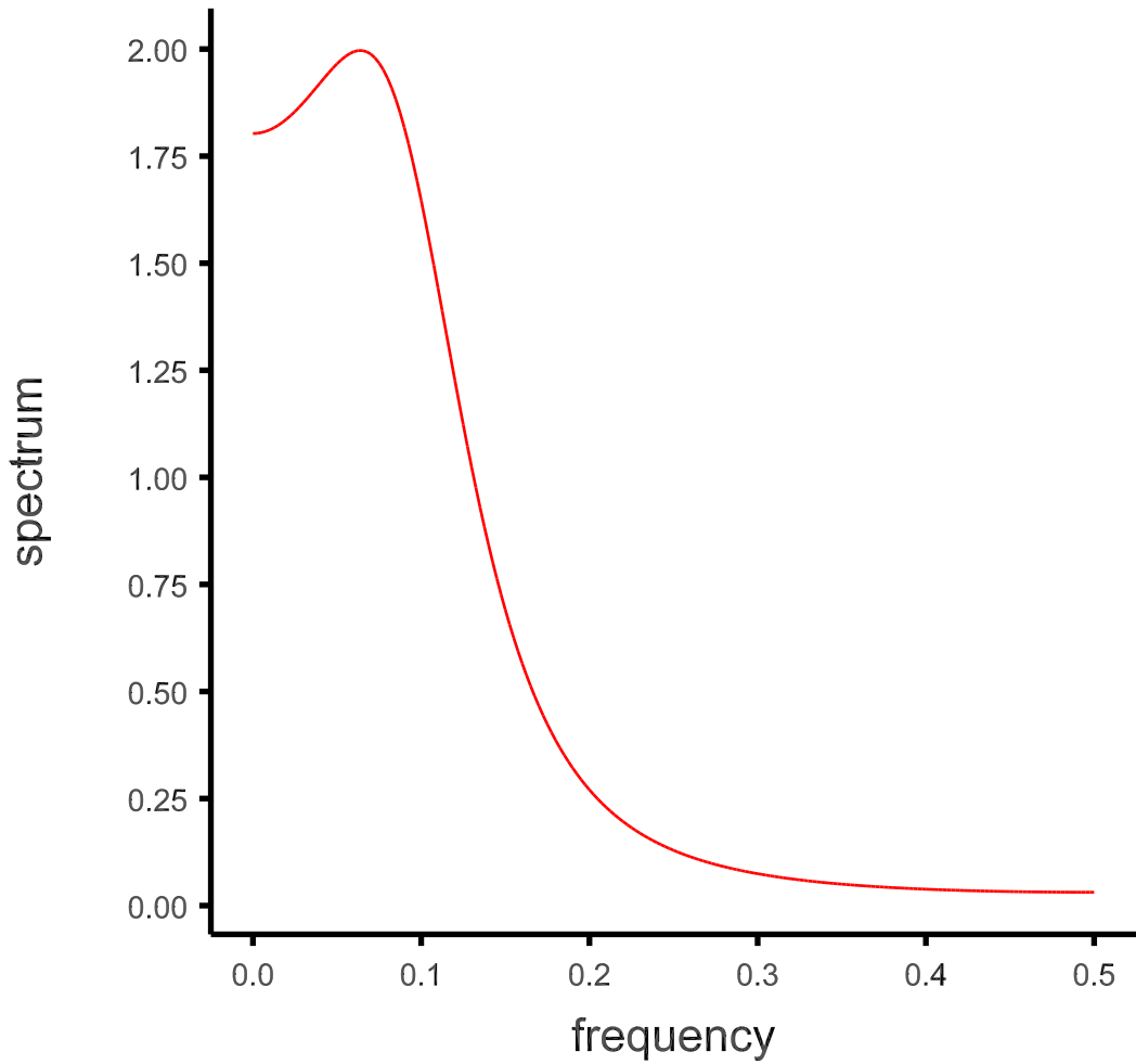
AR(2) model spectrum
