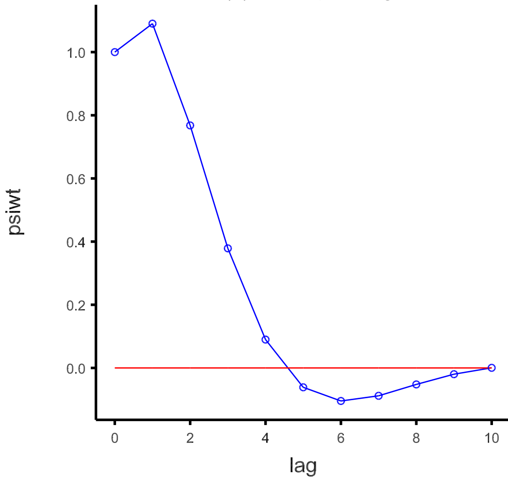
AR(2) model psi-weight
