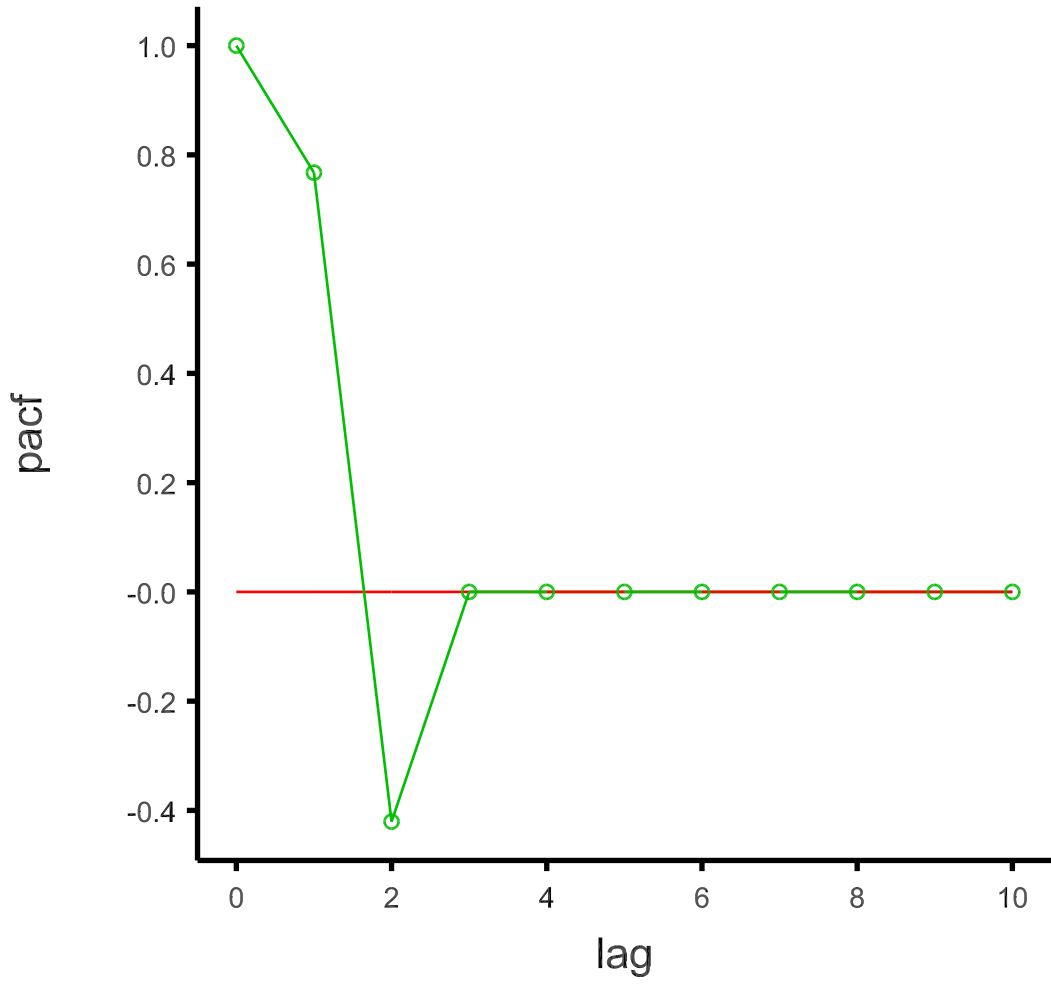
AR(2) model pacf
