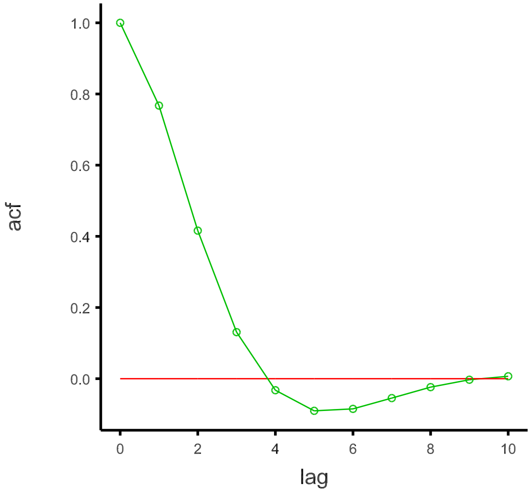
AR(2) model acf
