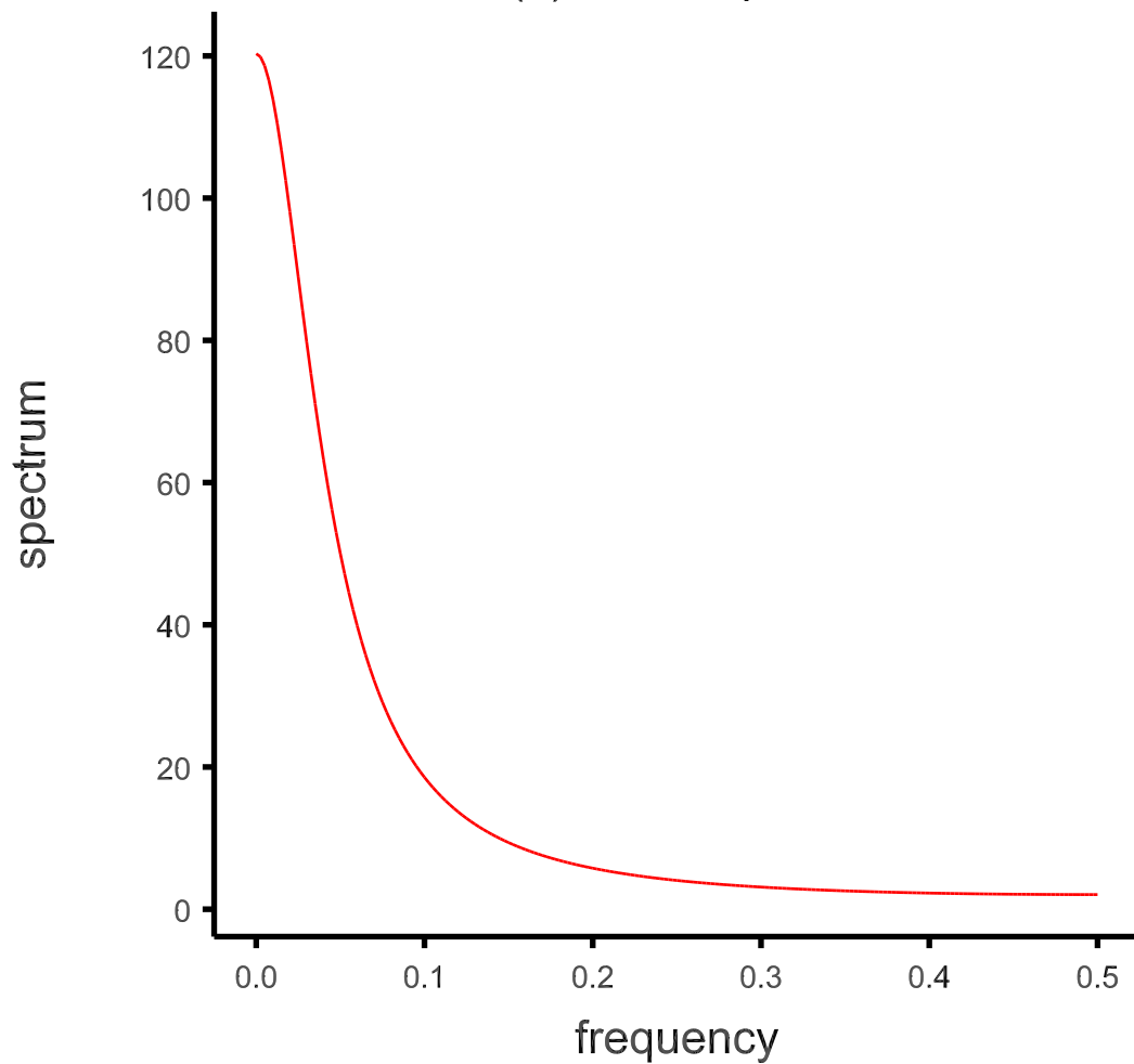
AR(1) model spectrum
