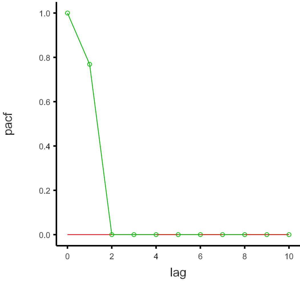
AR(1) model pacf
