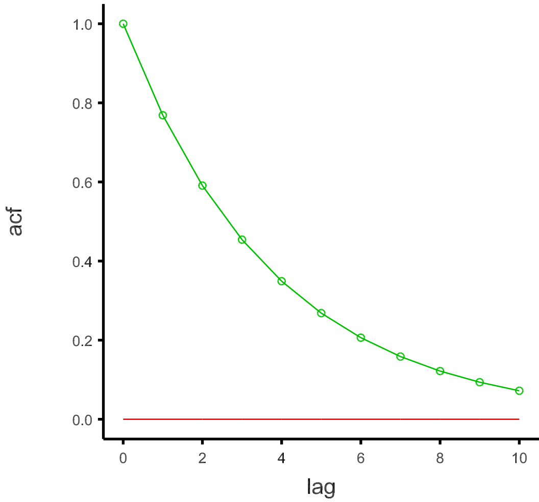
AR(1) model acf
