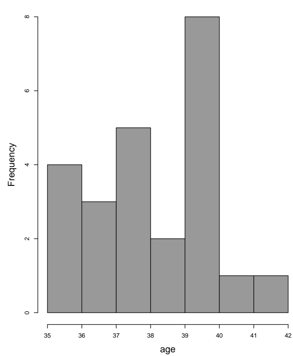
Histogram of age
