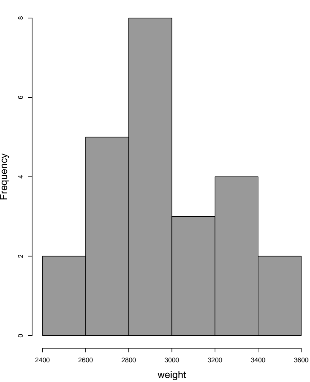
Histogram of weight
