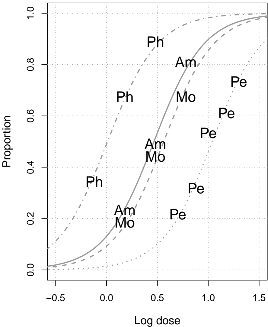
Main Effects Model
